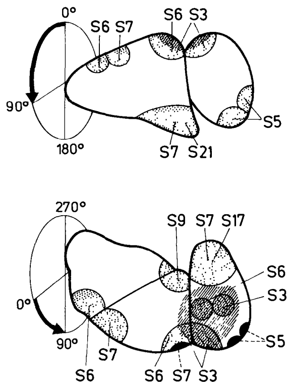
Fig.3. Presumptive localization of the eIF-2 binding site on the 40 S ribosomal subunit (///// ) and the position of the antigenic determinants of ribosomal proteins (●) upper level; (●) lower level of projection) as determined by immune electron microscopic studies ([8,9] and unpublished).
