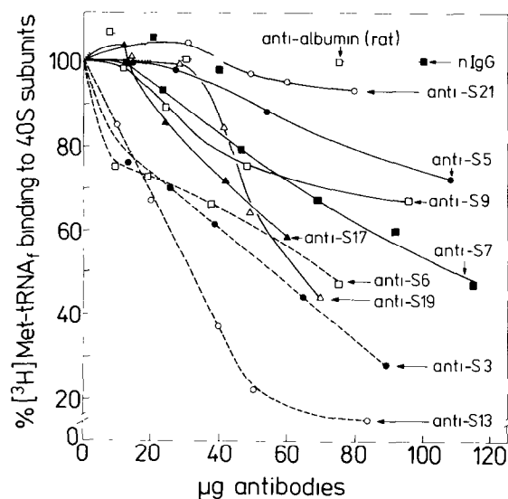
Fig.2. Inhibition of [ ^3\text{H} ]Met-tRNA f binding to small ribosomal subunits by antibodies against pure ribosomal proteins. eIF-2-dependent binding of [ ^3\text{H} ]Met-tRNA f to 40 S subunits in the presence of the indicated amounts of antibodies was assayed as in section 2. Each point demonstrates [ ^3\text{H} ]Met-tRNA f binding to the 40 S subunit in relation to the control experiment without antibodies. 100% corresponds to [ ^3\text{H} ]Met-tRNA f binding to 14 \mu\text{g} 40 S subunits over 1.5–2.0 pmol (nIgG, immunoglobulin G fraction from non-immune antiserum).
